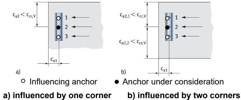
FIGURE 4-16: EXAMPLE OF AN ANCHOR CHANNEL LOADED IN SHEAR WITH ANCHORS:
